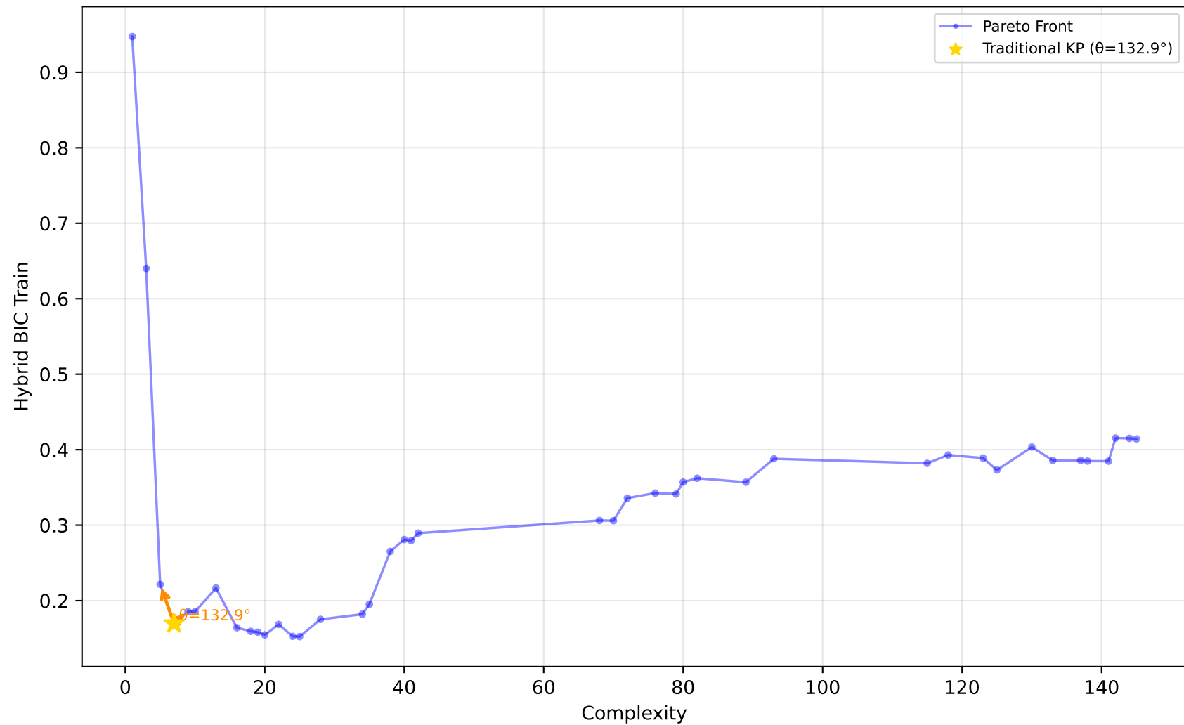
519_vinnie - Run 13 - MVP - Hybrid BIC Train \lambda_1=1.00, \lambda_2=0.00, \lambda_3=1.00 | Difficulty: 0.54 | Method: mckp
