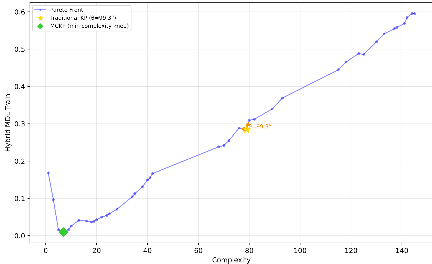
519_vinnie - Run 13 - MVP - Hybrid MDL Train \lambda_1=0.00, \lambda_2=0.10, \lambda_3=0.00 | Difficulty: 0.54 | Method: mckp
