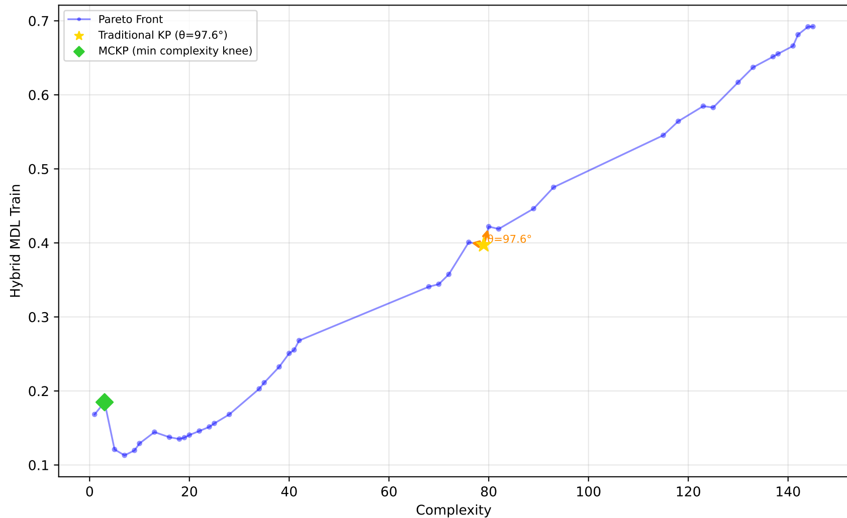
519_vinnie - Run 13 - MVP - Hybrid MDL Train \lambda_1=1.00, \lambda_2=0.00, \lambda_3=1.00 | Difficulty: 0.54 | Method: mckp
