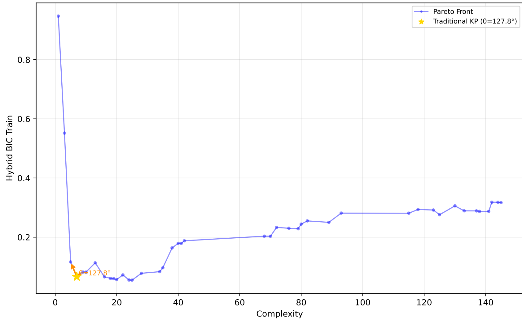
519_vinnie - Run 13 - SVP - Hybrid BIC Train \lambda_1=0.00, \lambda_2=0.00, \lambda_3=0.00 | Difficulty: 0.54 | Method: mckp
