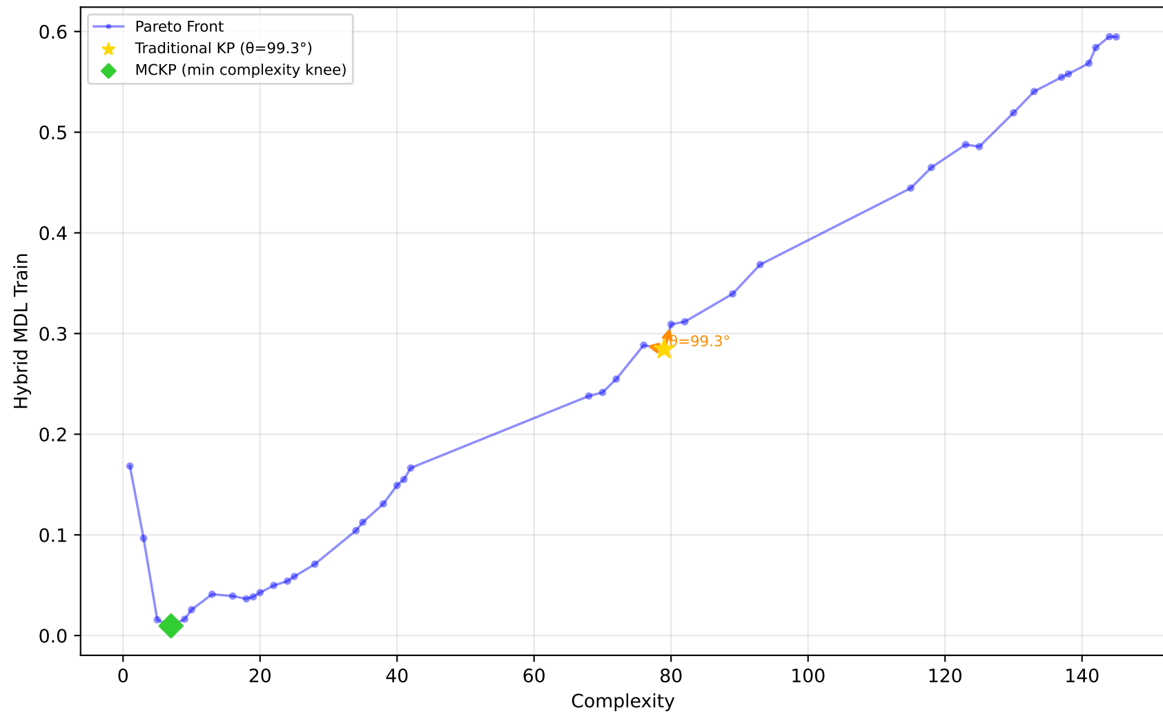
519_vinnie - Run 13 - SVP - Hybrid MDL Train \lambda_1=0.00, \lambda_2=0.00, \lambda_3=0.00 | Difficulty: 0.54 | Method: mckp
