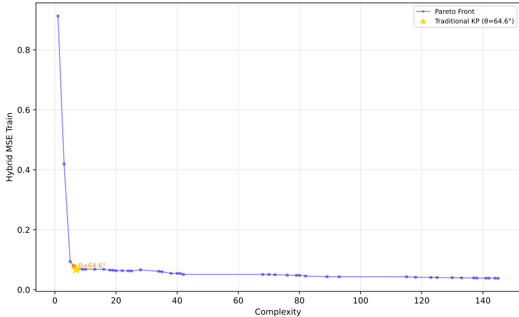
519_vinnie - Run 13 - SVP - Hybrid MSE Train \lambda_1=0.00, \lambda_2=0.00, \lambda_3=0.00 | Difficulty: 0.54 | Method: mckp
