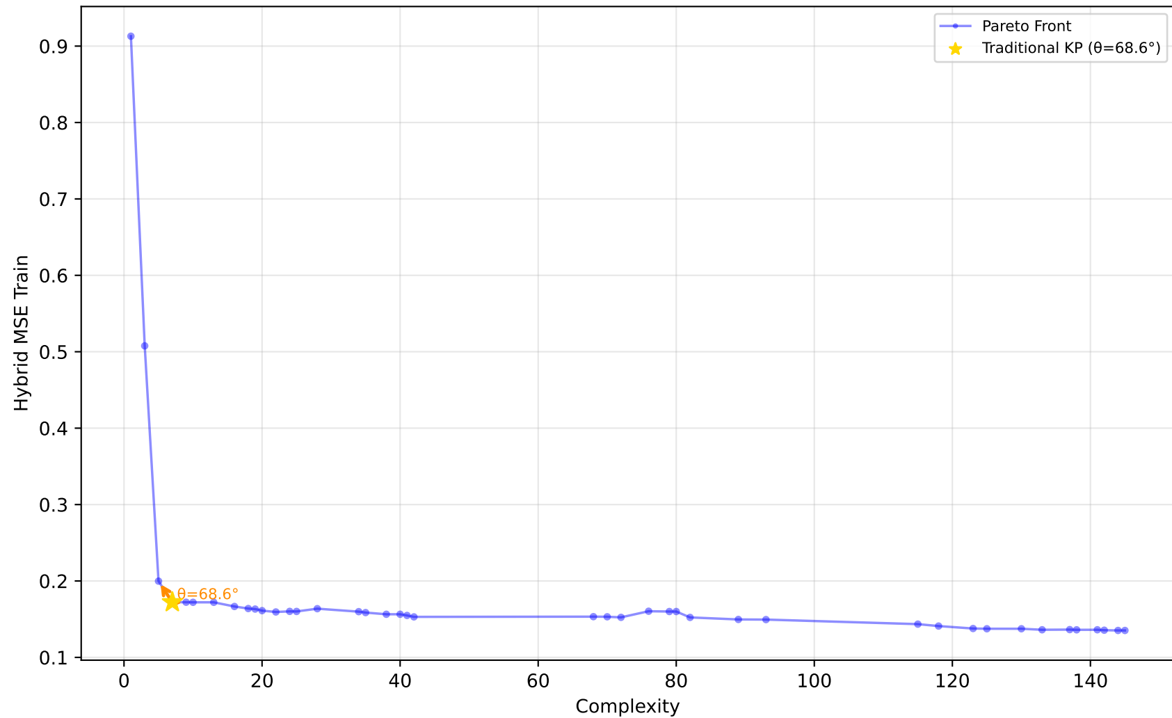
519_vinnie - Run 13 - SVP - Hybrid MSE Train \lambda_1=1.00, \lambda_2=1.00, \lambda_3=1.00 | Difficulty: 0.54 | Method: mckp
