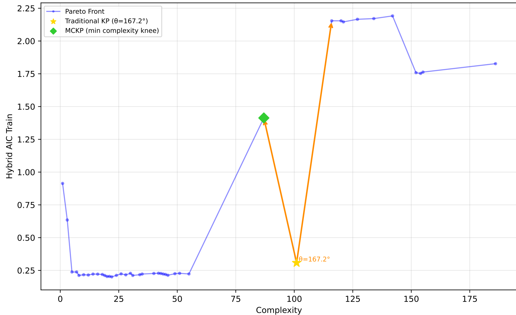
519_vinnie - Run 14 - MVP - Hybrid AIC Train \lambda_1=1.00, \lambda_2=0.00, \lambda_3=1.00 | Difficulty: 0.45 | Method: mckp
