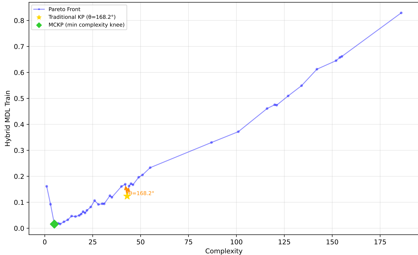
519_vinnie - Run 14 - MVP - Hybrid MDL Train \lambda_1=0.00, \lambda_2=0.10, \lambda_3=0.00 | Difficulty: 0.45 | Method: mckp
