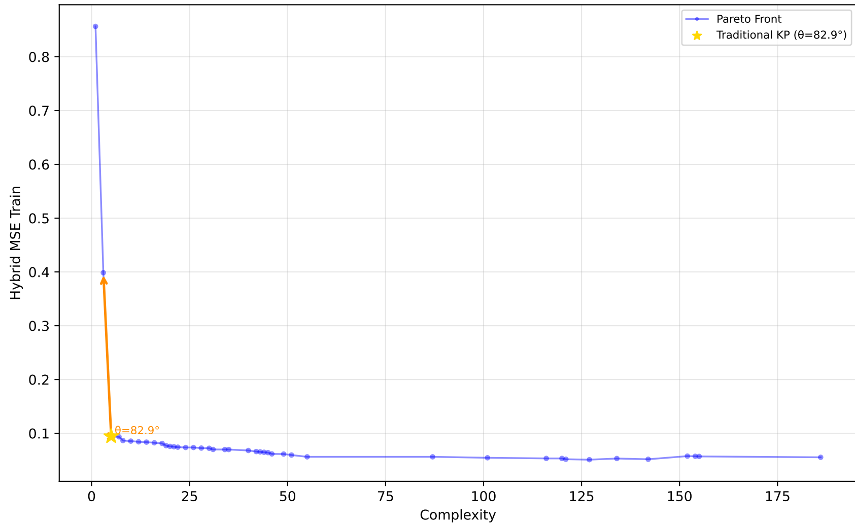
519_vinnie - Run 14 - MVP - Hybrid MSE Train \lambda_1=0.00, \lambda_2=0.10, \lambda_3=0.00 | Difficulty: 0.45 | Method: mckp
