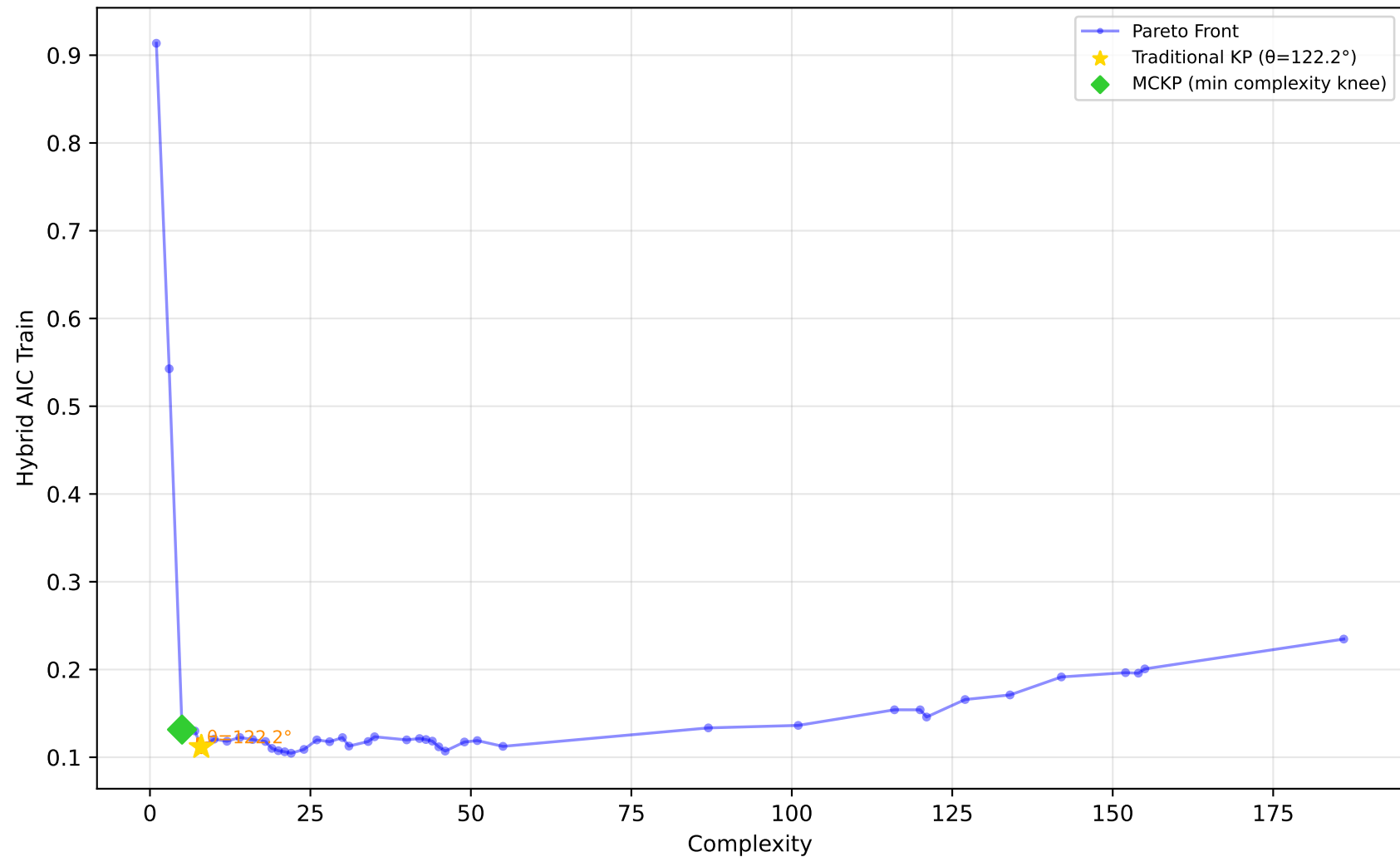
519_vinnie - Run 14 - SVP - Hybrid AIC Train \lambda_1=0.00, \lambda_2=0.00, \lambda_3=0.00 | Difficulty: 0.45 | Method: mckp
