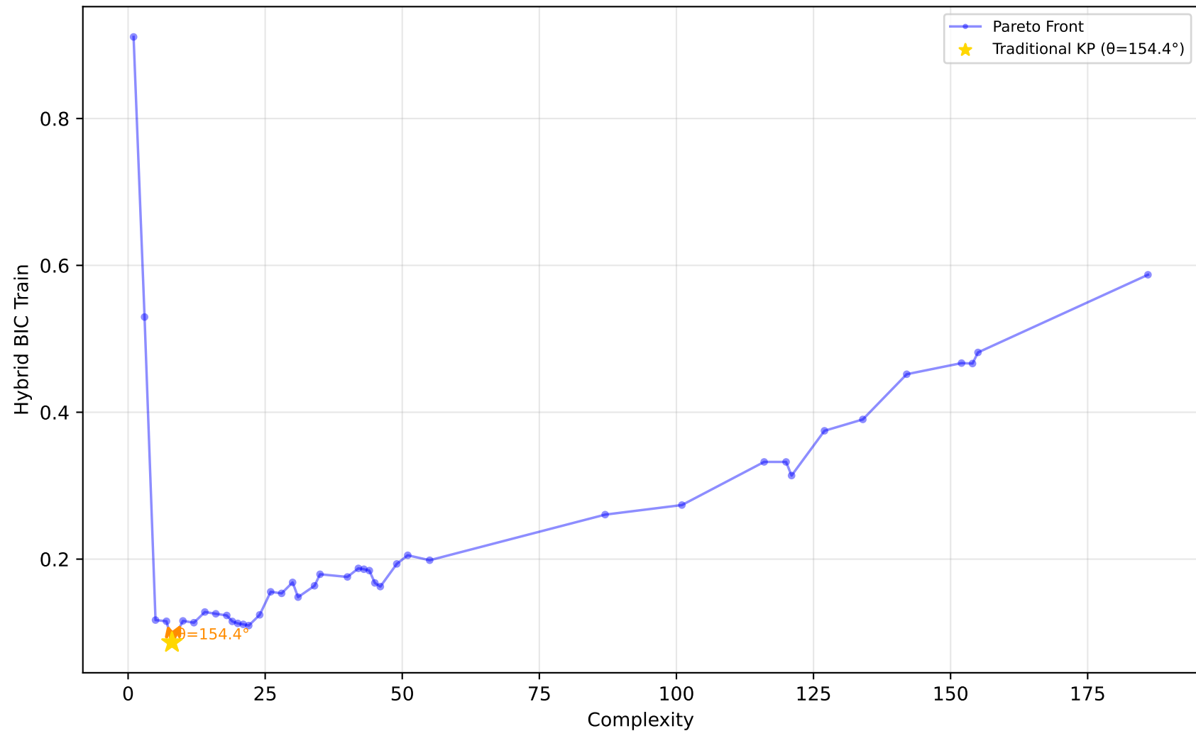
519_vinnie - Run 14 - SVP - Hybrid BIC Train \lambda_1=0.00, \lambda_2=0.00, \lambda_3=0.00 | Difficulty: 0.45 | Method: mckp
