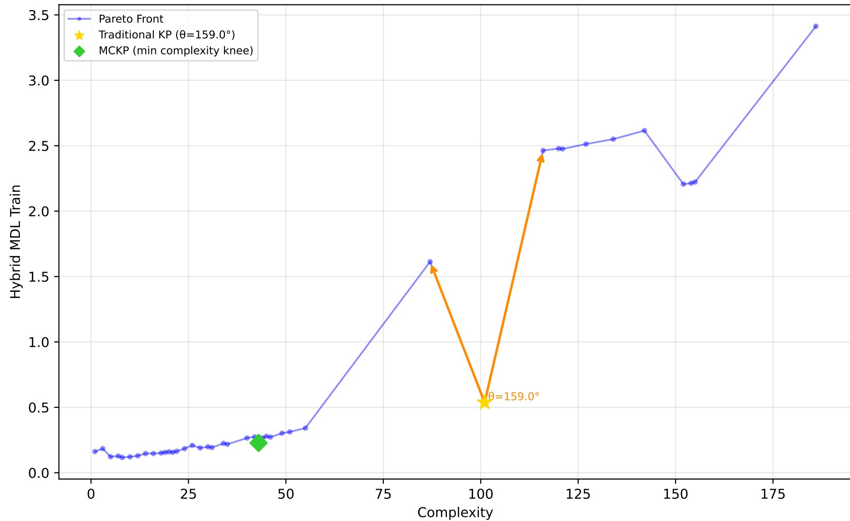
519_vinnie - Run 14 - SVP - Hybrid MDL Train \lambda_1=1.00, \lambda_2=1.00, \lambda_3=1.00 | Difficulty: 0.45 | Method: mckp
