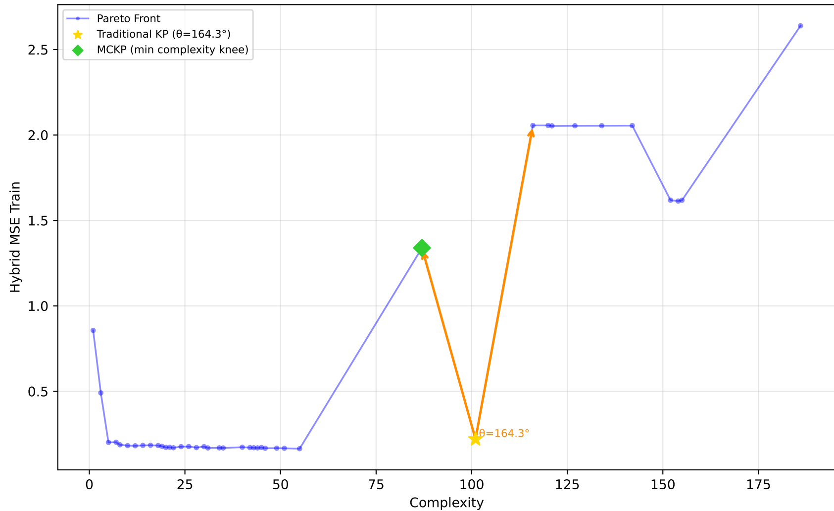
519_vinnie - Run 14 - SVP - Hybrid MSE Train \lambda_1=1.00, \lambda_2=1.00, \lambda_3=1.00 | Difficulty: 0.45 | Method: mckp
