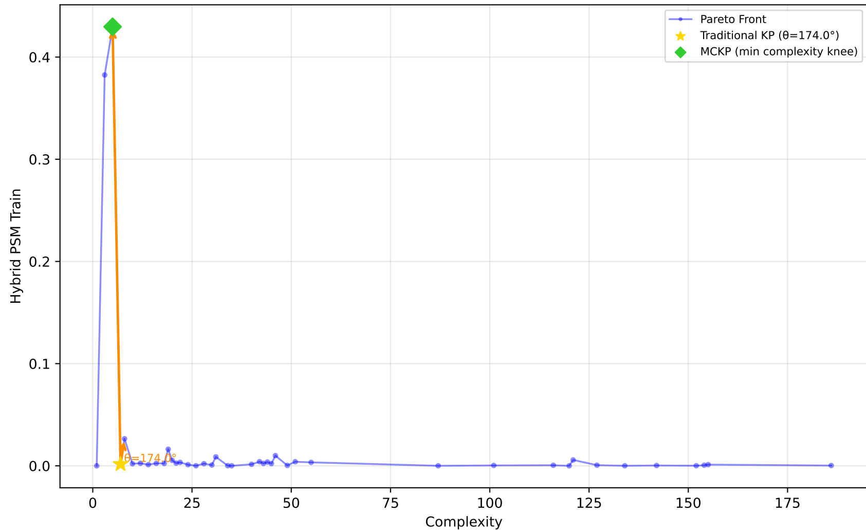
519_vinnie - Run 14 - SVP - Hybrid PSM Train \lambda_1=0.00, \lambda_2=0.00, \lambda_3=0.00 | Difficulty: 0.45 | Method: mckp
