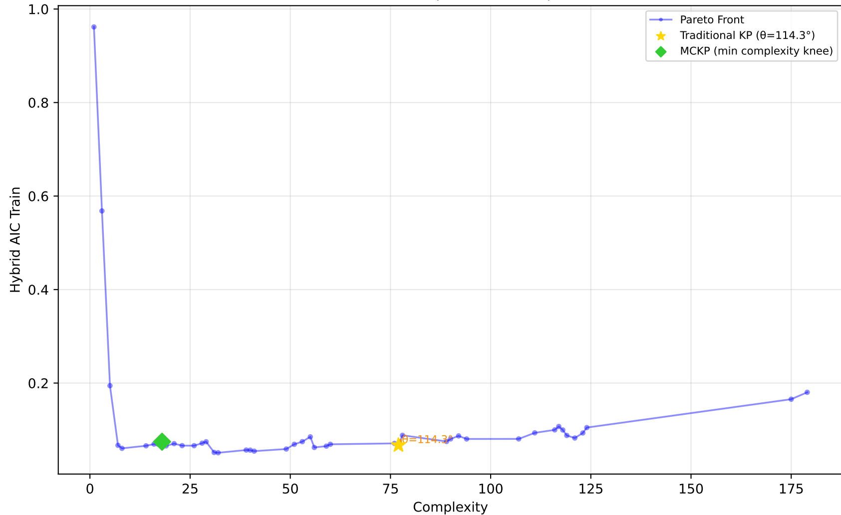
519_vinnie - Run 15 - MVP - Hybrid AIC Train \lambda_1=0.00, \lambda_2=0.10, \lambda_3=0.00 | Difficulty: 0.49 | Method: mckp
