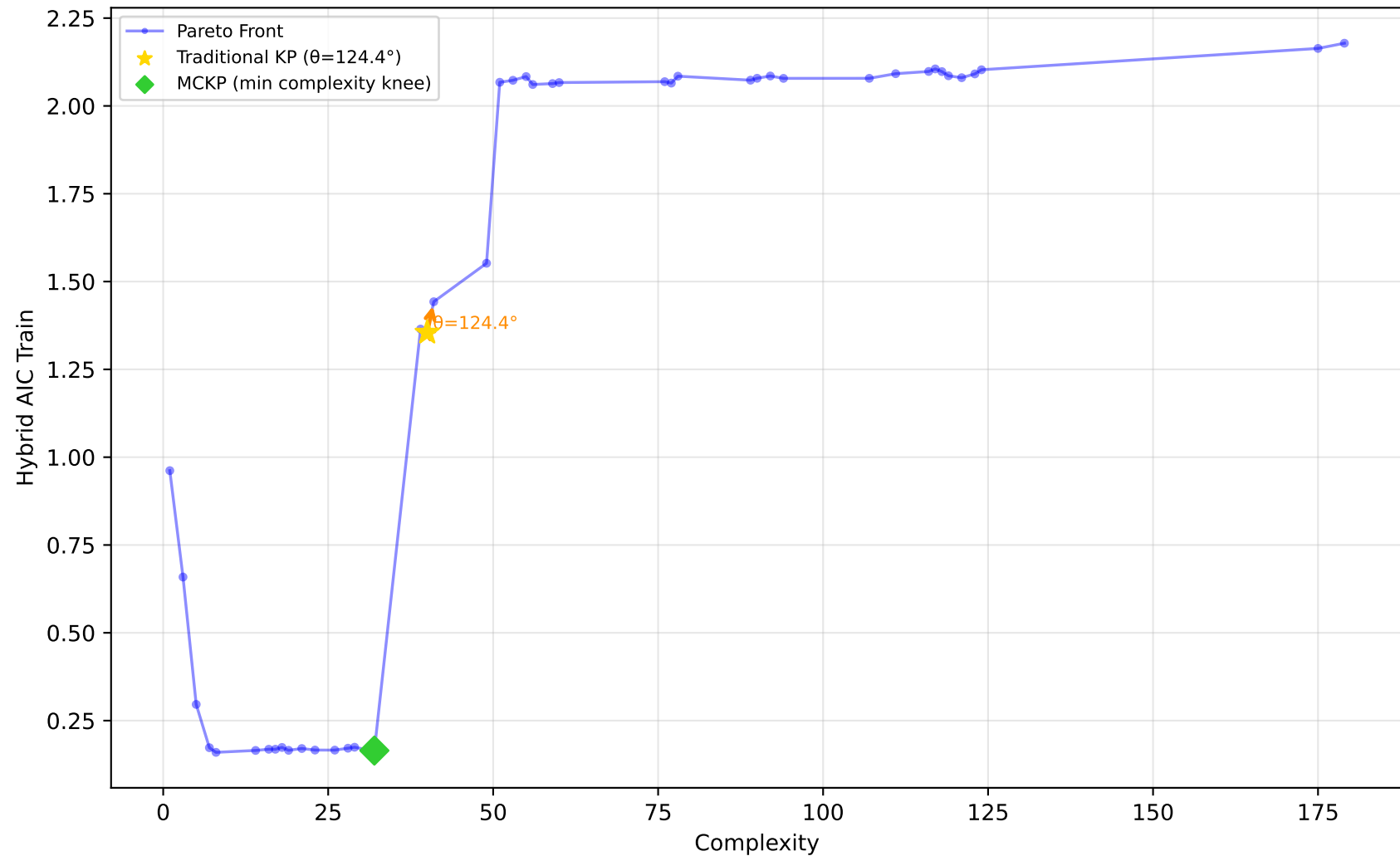
519_vinnie - Run 15 - MVP - Hybrid AIC Train \lambda_1=1.00, \lambda_2=0.00, \lambda_3=1.00 | Difficulty: 0.49 | Method: mckp
