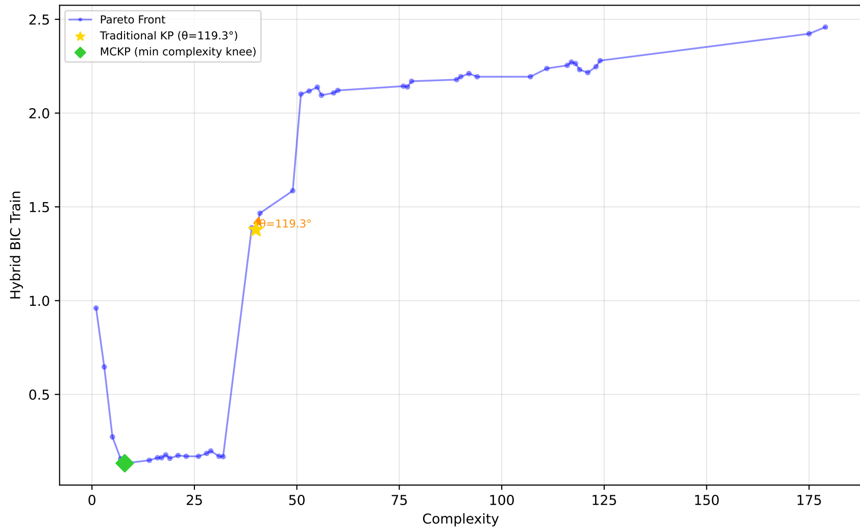
519_vinnie - Run 15 - MVP - Hybrid BIC Train \lambda_1=1.00, \lambda_2=0.00, \lambda_3=1.00 | Difficulty: 0.49 | Method: mckp
