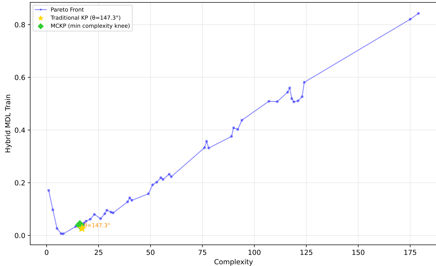
519_vinnie - Run 15 - MVP - Hybrid MDL Train \lambda_1=0.00, \lambda_2=0.10, \lambda_3=0.00 | Difficulty: 0.49 | Method: mckp
