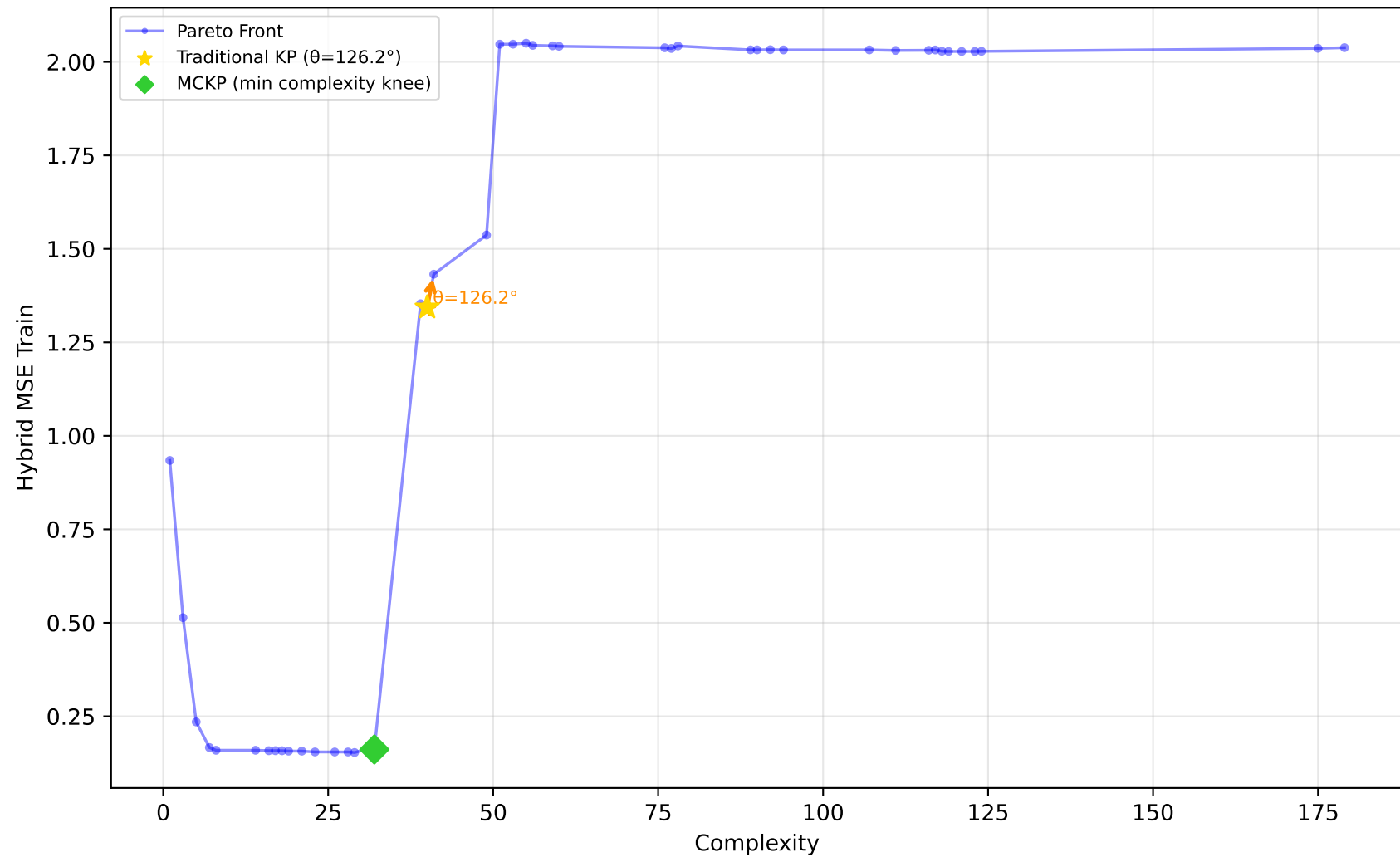
519_vinnie - Run 15 - MVP - Hybrid MSE Train \lambda_1=1.00, \lambda_2=0.00, \lambda_3=1.00 | Difficulty: 0.49 | Method: mckp
