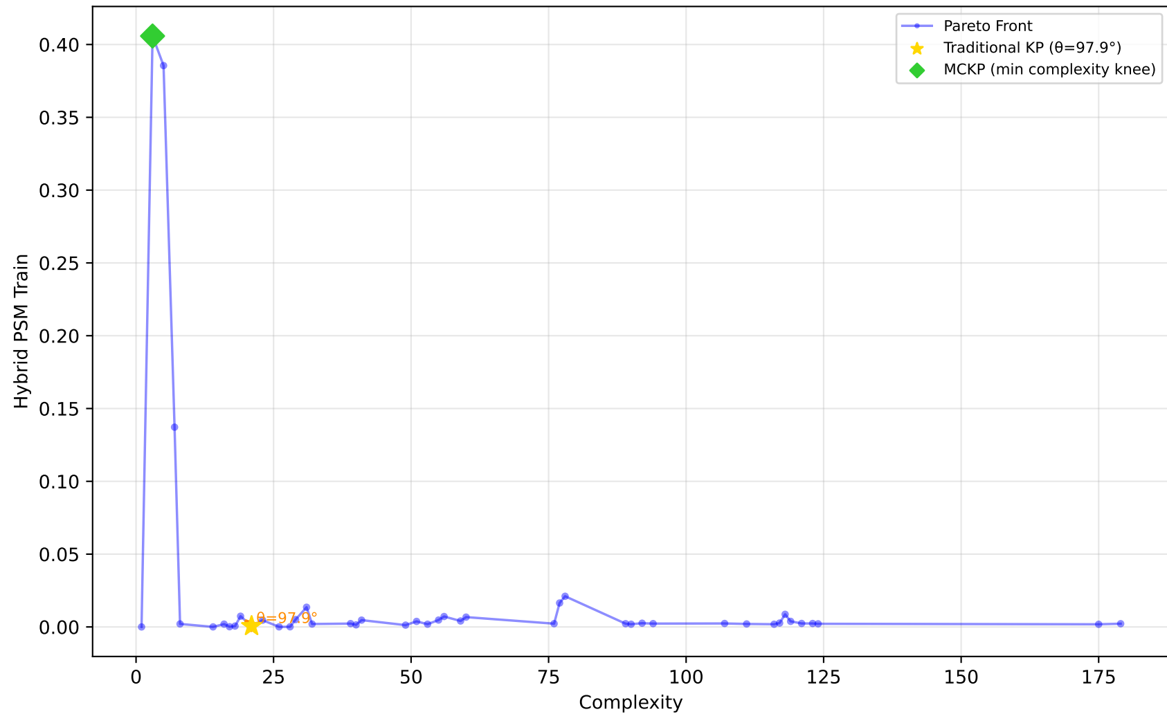
519_vinnie - Run 15 - MVP - Hybrid PSM Train \lambda_1=0.00, \lambda_2=0.10, \lambda_3=0.00 | Difficulty: 0.49 | Method: mckp
