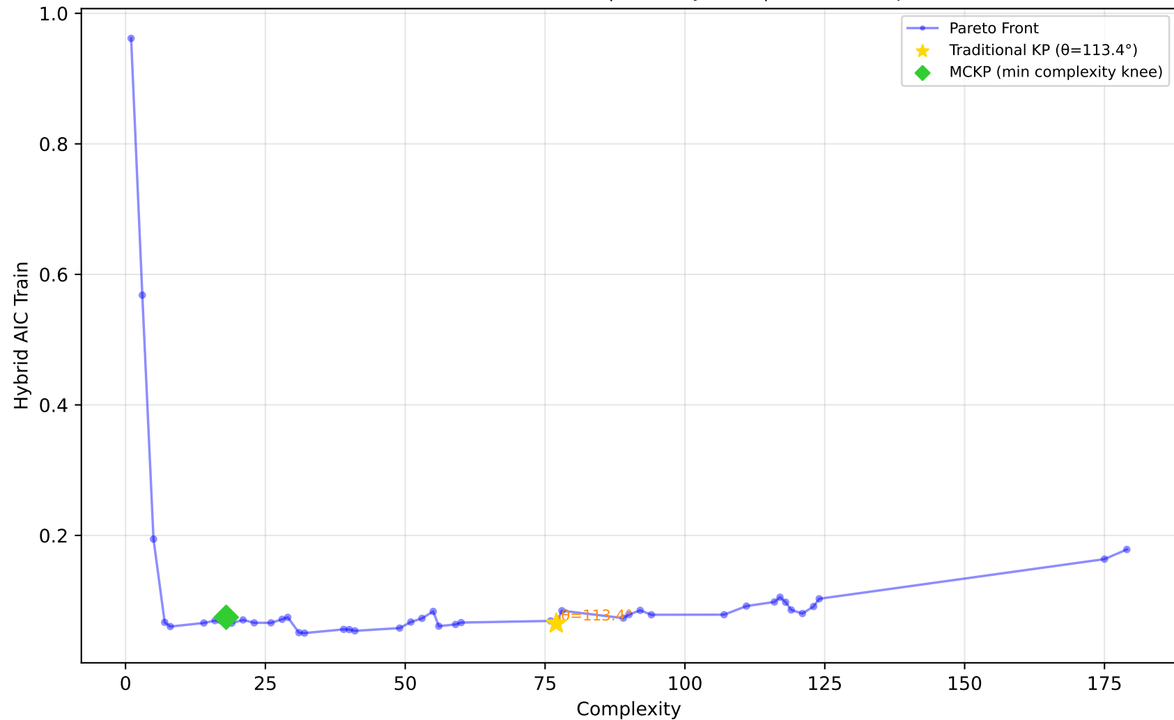
519_vinnie - Run 15 - SVP - Hybrid AIC Train \lambda_1=0.00, \lambda_2=0.00, \lambda_3=0.00 | Difficulty: 0.49 | Method: mckp
