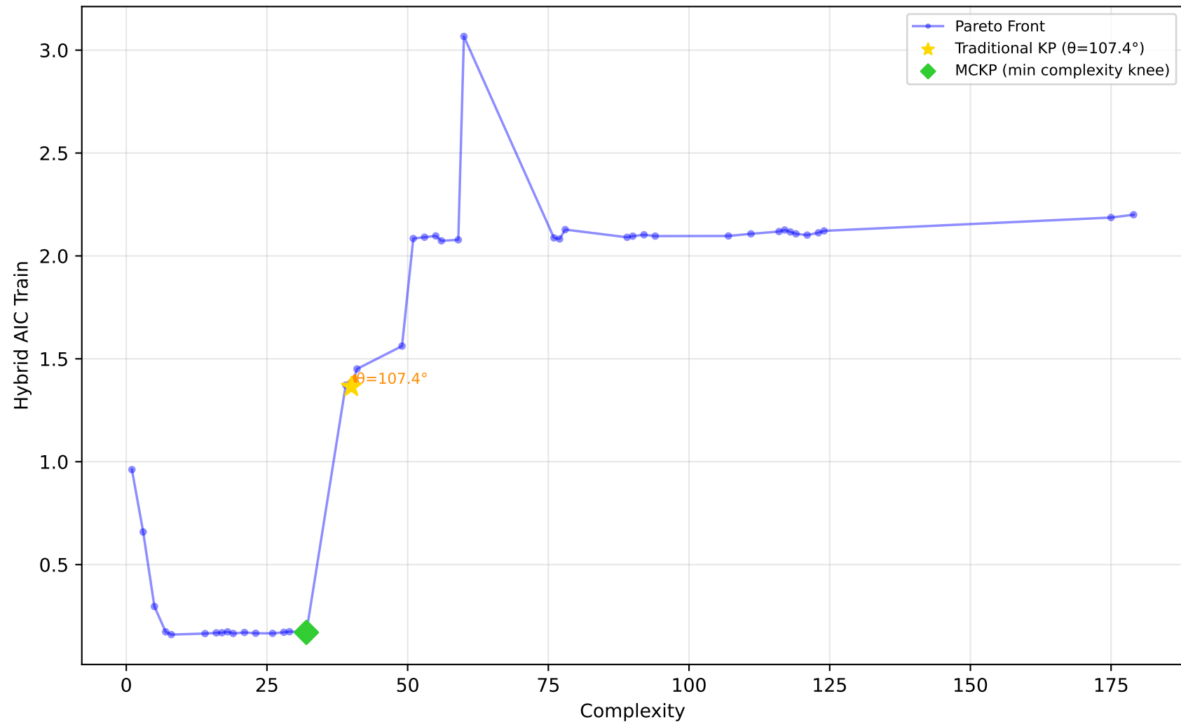
519_vinnie - Run 15 - SVP - Hybrid AIC Train \lambda_1=1.00, \lambda_2=1.00, \lambda_3=1.00 | Difficulty: 0.49 | Method: mckp
