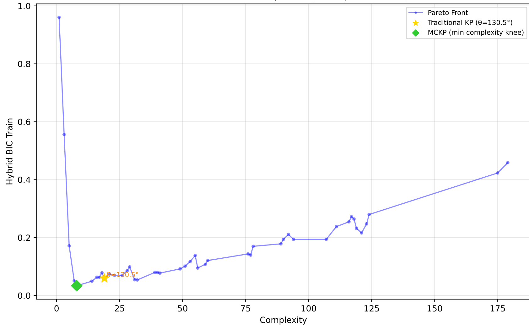
519_vinnie - Run 15 - SVP - Hybrid BIC Train \lambda_1=0.00, \lambda_2=0.00, \lambda_3=0.00 | Difficulty: 0.49 | Method: mckp
