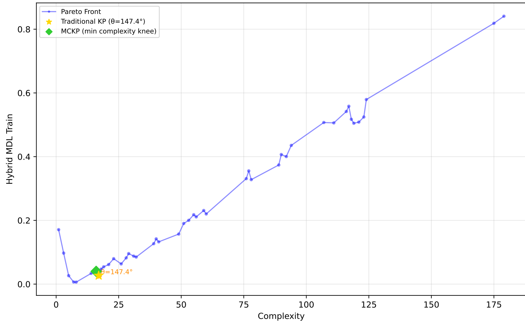
519_vinnie - Run 15 - SVP - Hybrid MDL Train \lambda_1=0.00, \lambda_2=0.00, \lambda_3=0.00 | Difficulty: 0.49 | Method: mckp
