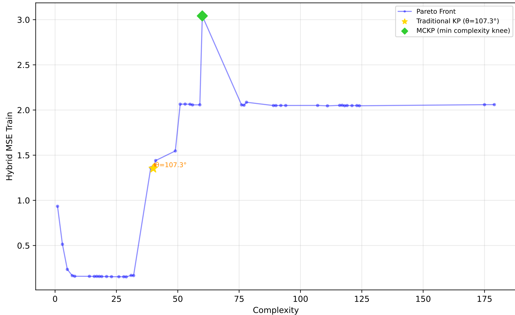
519_vinnie - Run 15 - SVP - Hybrid MSE Train \lambda_1=1.00, \lambda_2=1.00, \lambda_3=1.00 | Difficulty: 0.49 | Method: mckp
