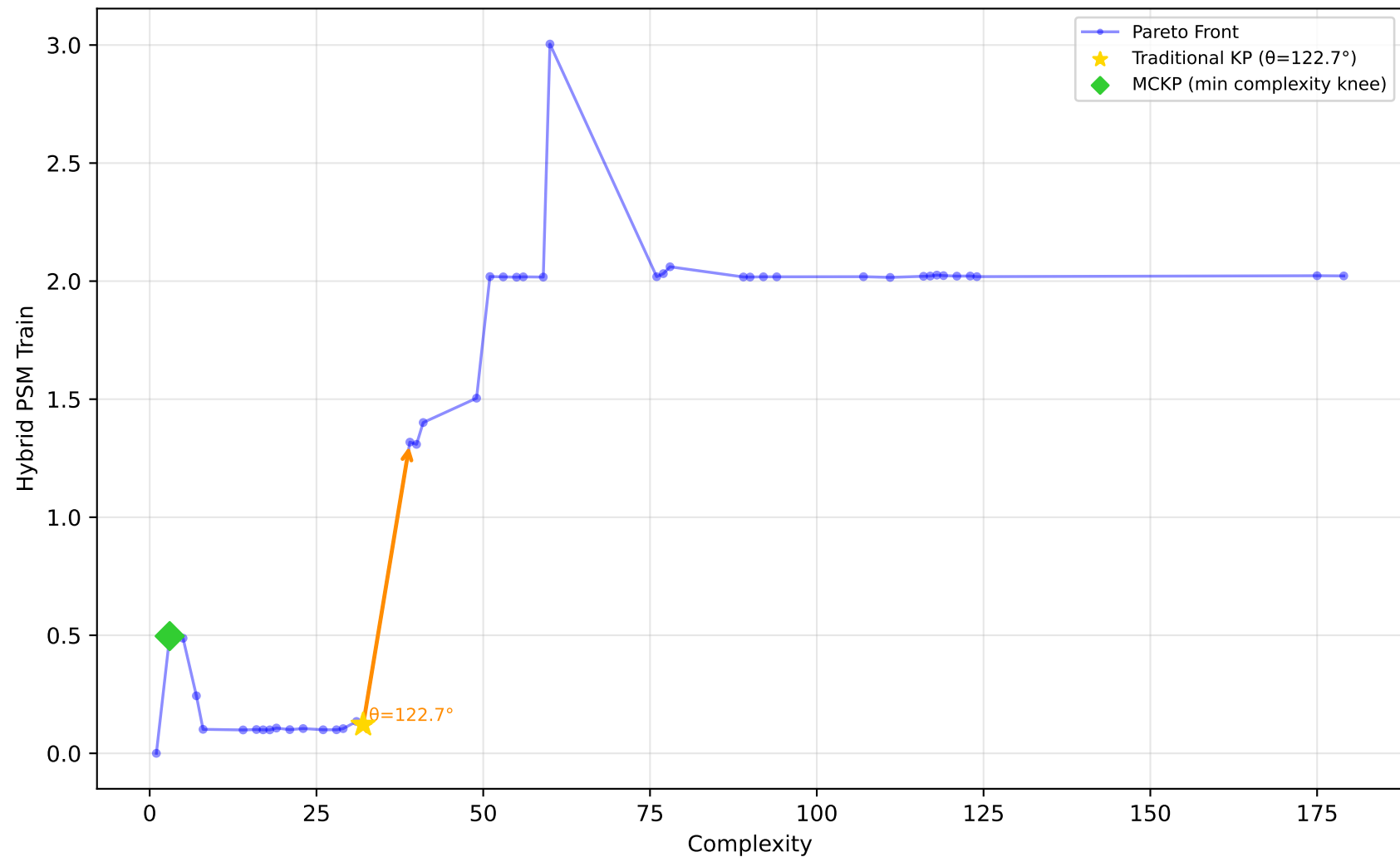
519_vinnie - Run 15 - SVP - Hybrid PSM Train \lambda_1=1.00, \lambda_2=1.00, \lambda_3=1.00 | Difficulty: 0.49 | Method: mckp
