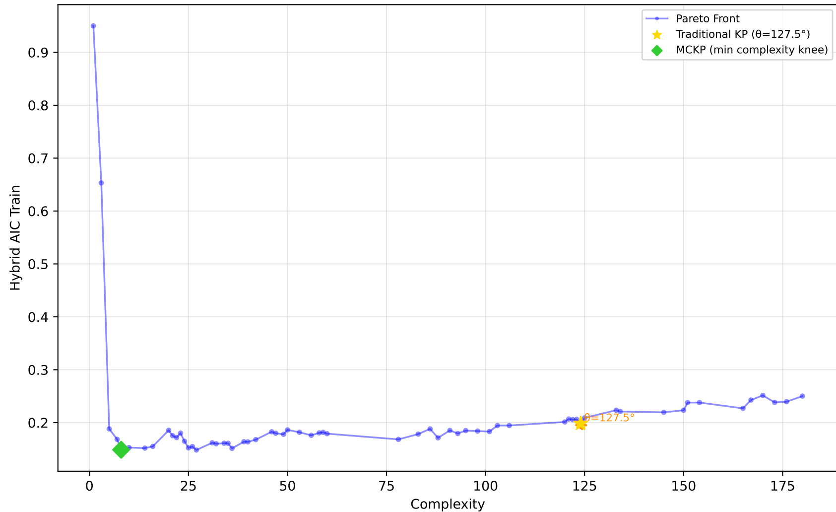
519_vinnie - Run 16 - MVP - Hybrid AIC Train \lambda_1=1.00, \lambda_2=0.00, \lambda_3=1.00 | Difficulty: 0.29 | Method: mckp
