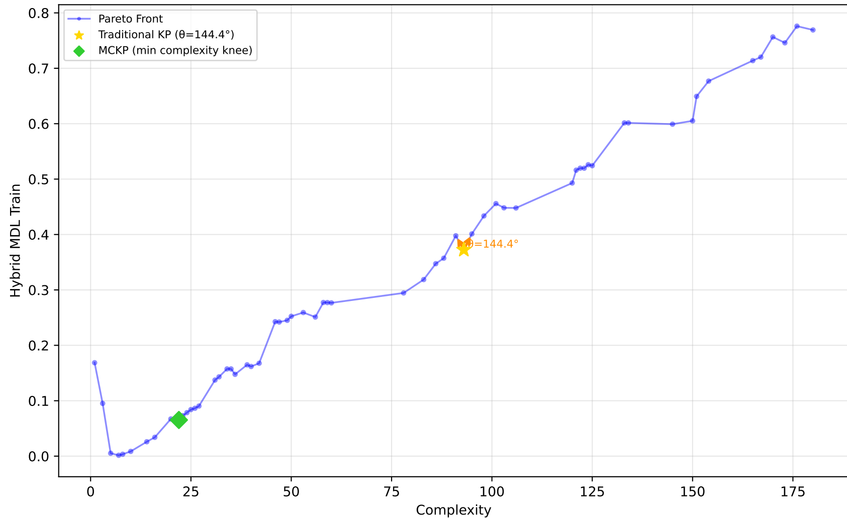
519_vinnie - Run 16 - MVP - Hybrid MDL Train \lambda_1=0.00, \lambda_2=0.10, \lambda_3=0.00 | Difficulty: 0.29 | Method: mckp
