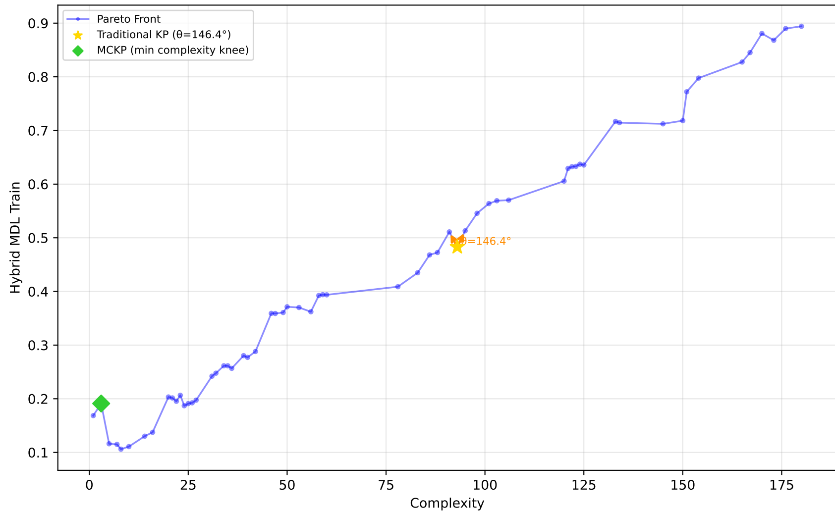
519_vinnie - Run 16 - MVP - Hybrid MDL Train \lambda_1=1.00, \lambda_2=0.00, \lambda_3=1.00 | Difficulty: 0.29 | Method: mckp
