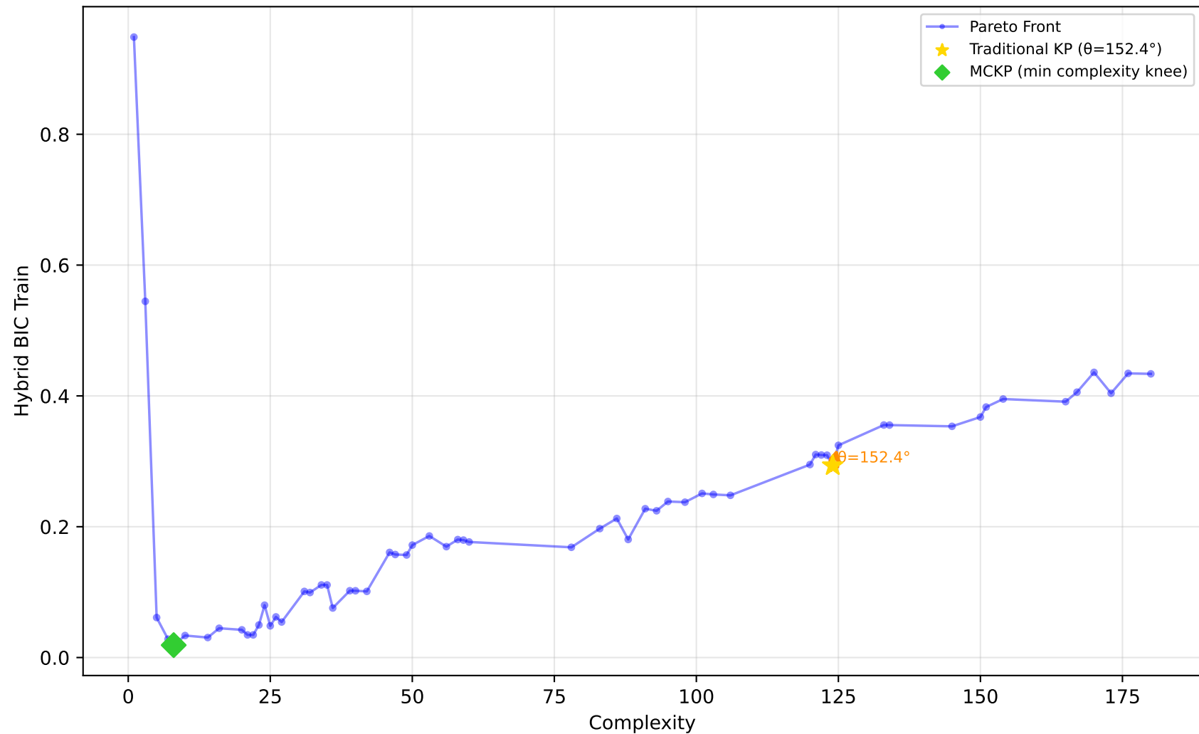
519_vinnie - Run 16 - SVP - Hybrid BIC Train \lambda_1=0.00, \lambda_2=0.00, \lambda_3=0.00 | Difficulty: 0.29 | Method: mckp
