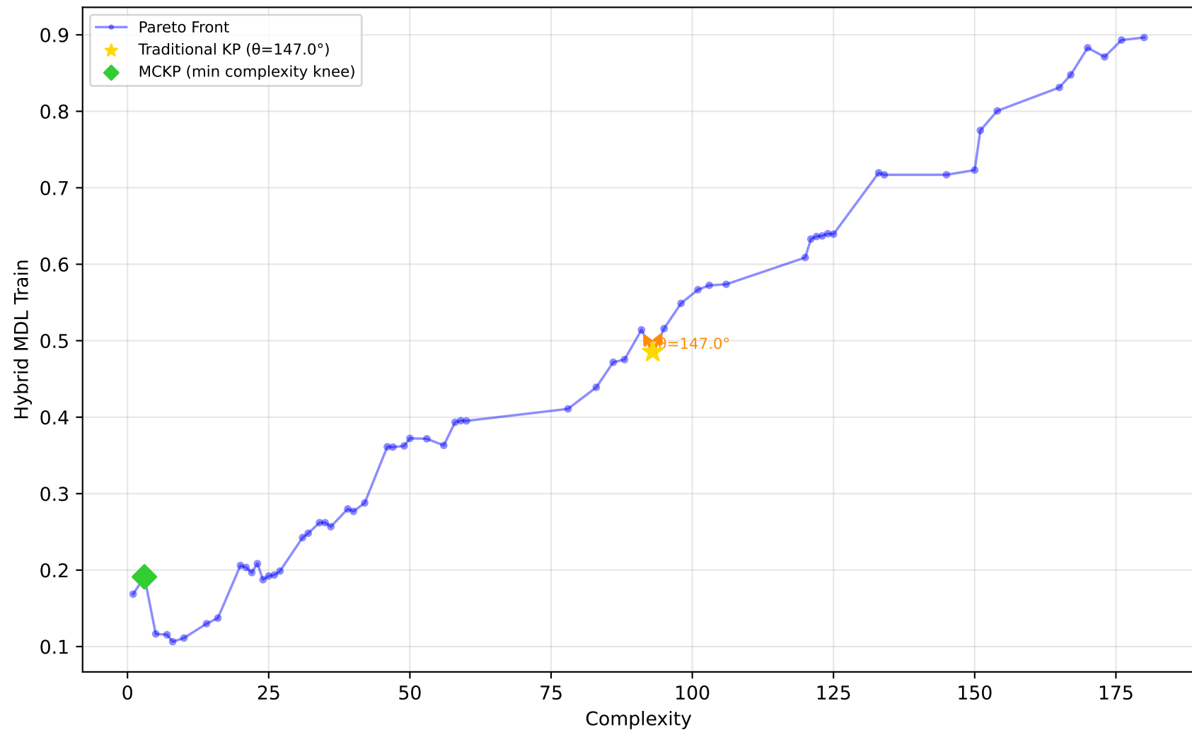
519_vinnie - Run 16 - SVP - Hybrid MDL Train \lambda_1=1.00, \lambda_2=1.00, \lambda_3=1.00 | Difficulty: 0.29 | Method: mckp
