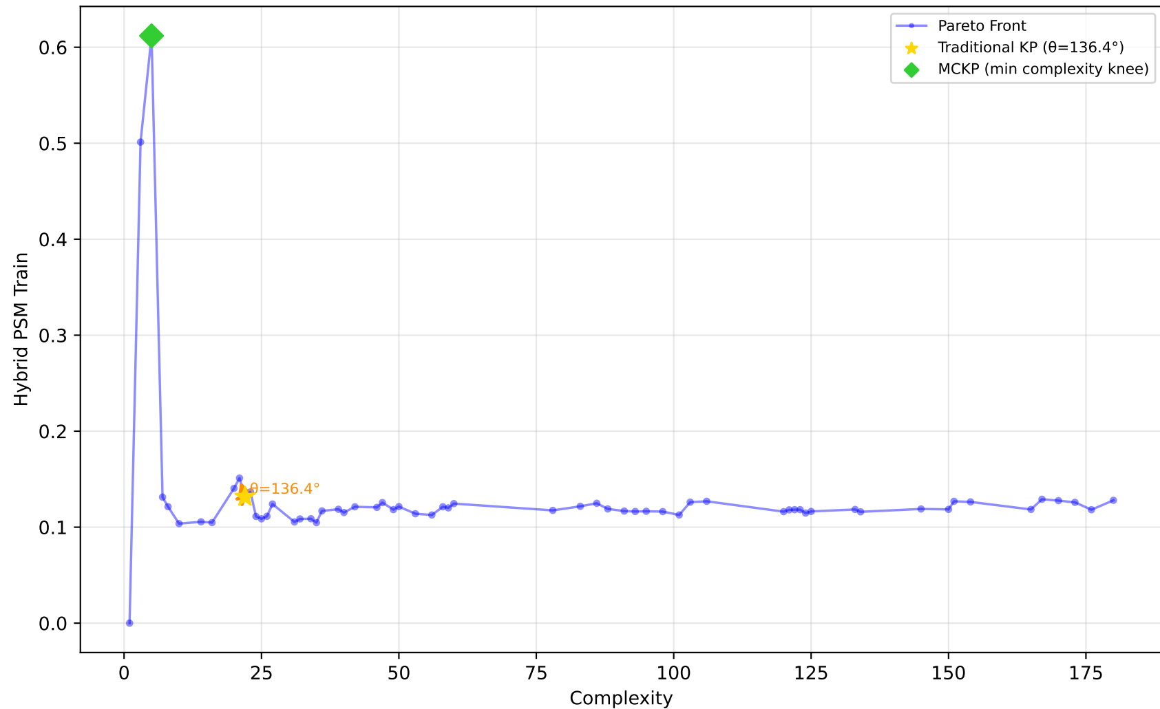
519_vinnie - Run 16 - SVP - Hybrid PSM Train \lambda_1=1.00, \lambda_2=1.00, \lambda_3=1.00 | Difficulty: 0.29 | Method: mckp
