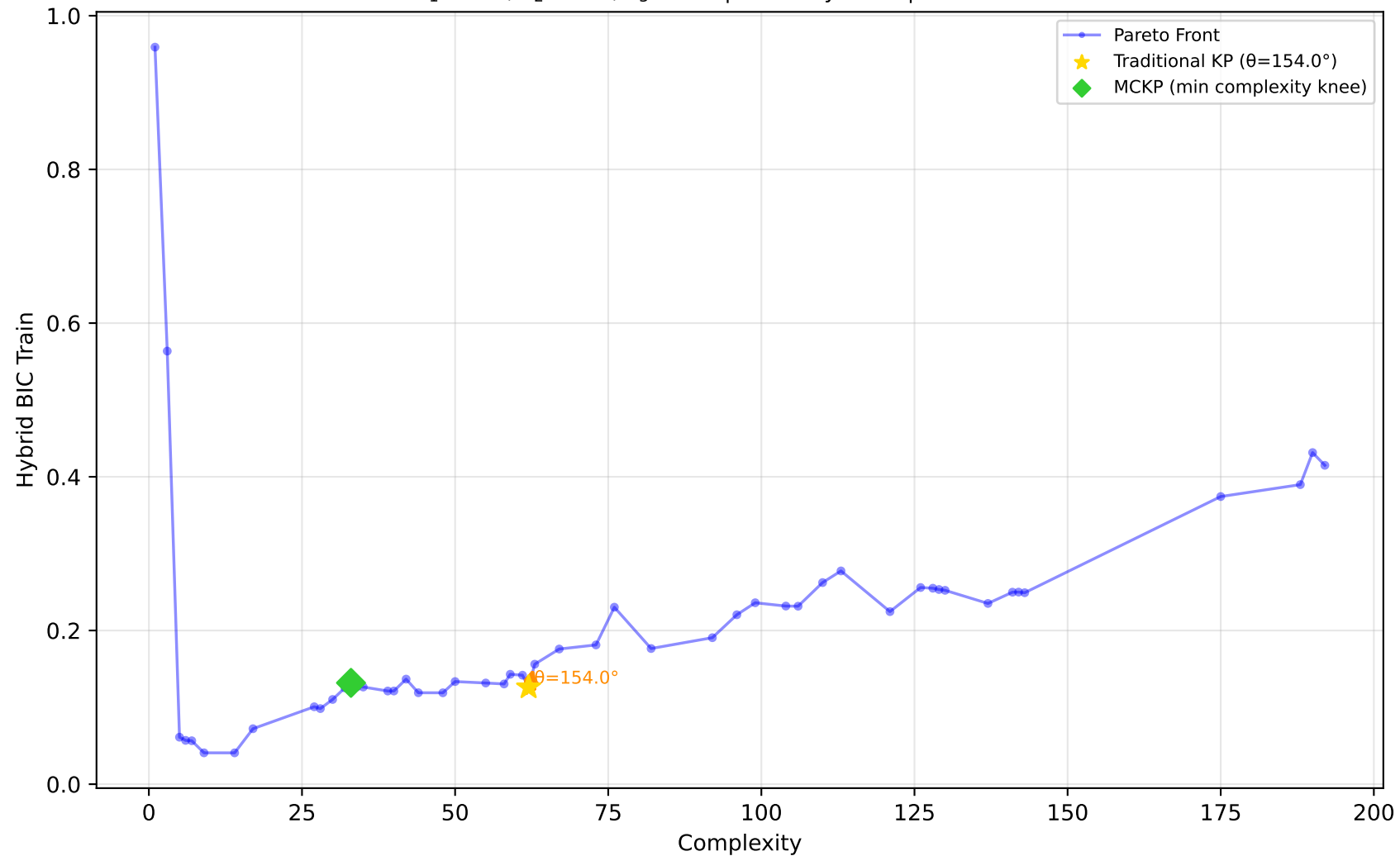
519_vinnie - Run 17 - MVP - Hybrid BIC Train \lambda_1=0.00, \lambda_2=0.10, \lambda_3=0.00 | Difficulty: 0.85 | Method: hmr
