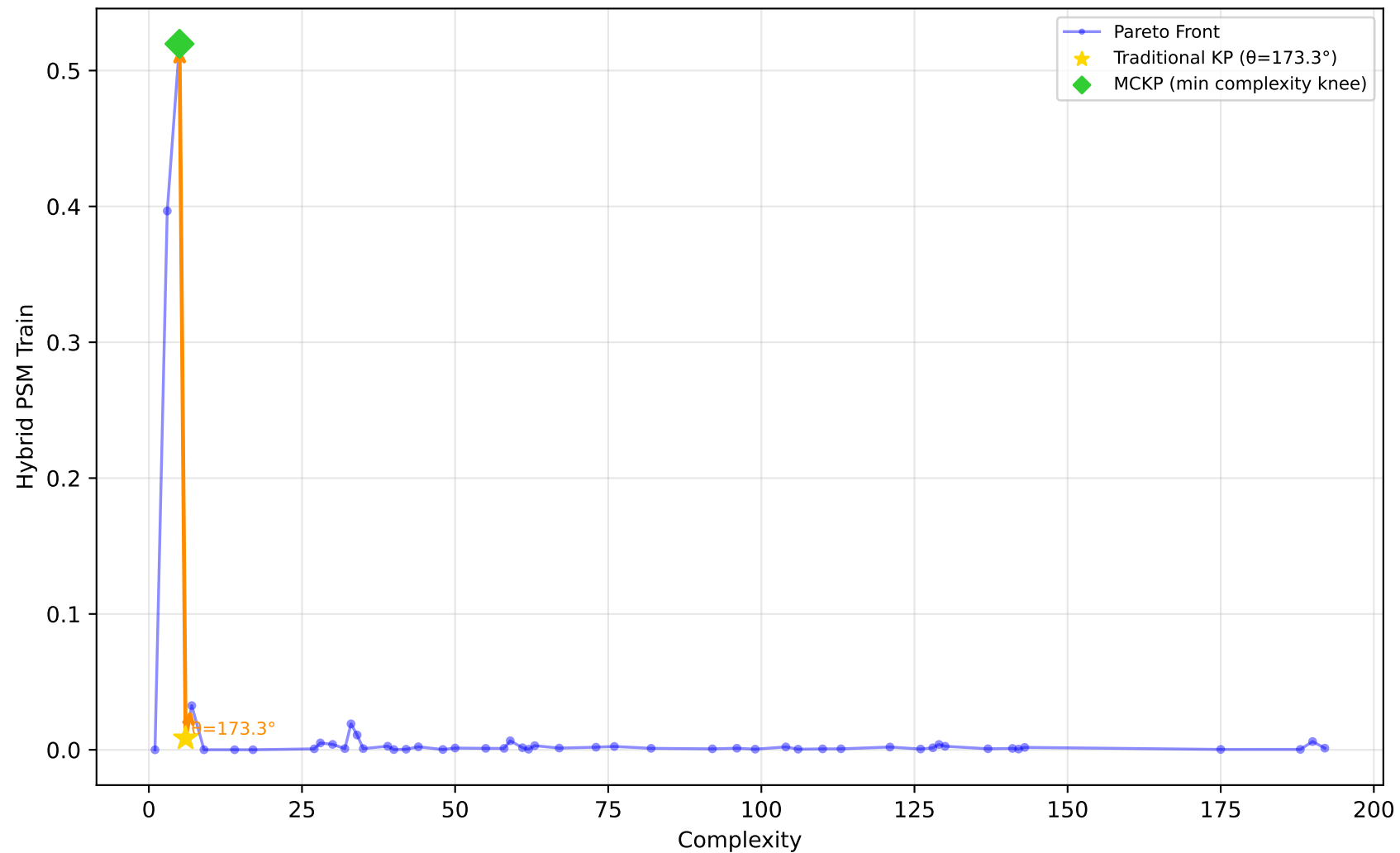
519_vinnie - Run 17 - MVP - Hybrid PSM Train \lambda_1=0.00, \lambda_2=0.10, \lambda_3=0.00 | Difficulty: 0.85 | Method: hmr
