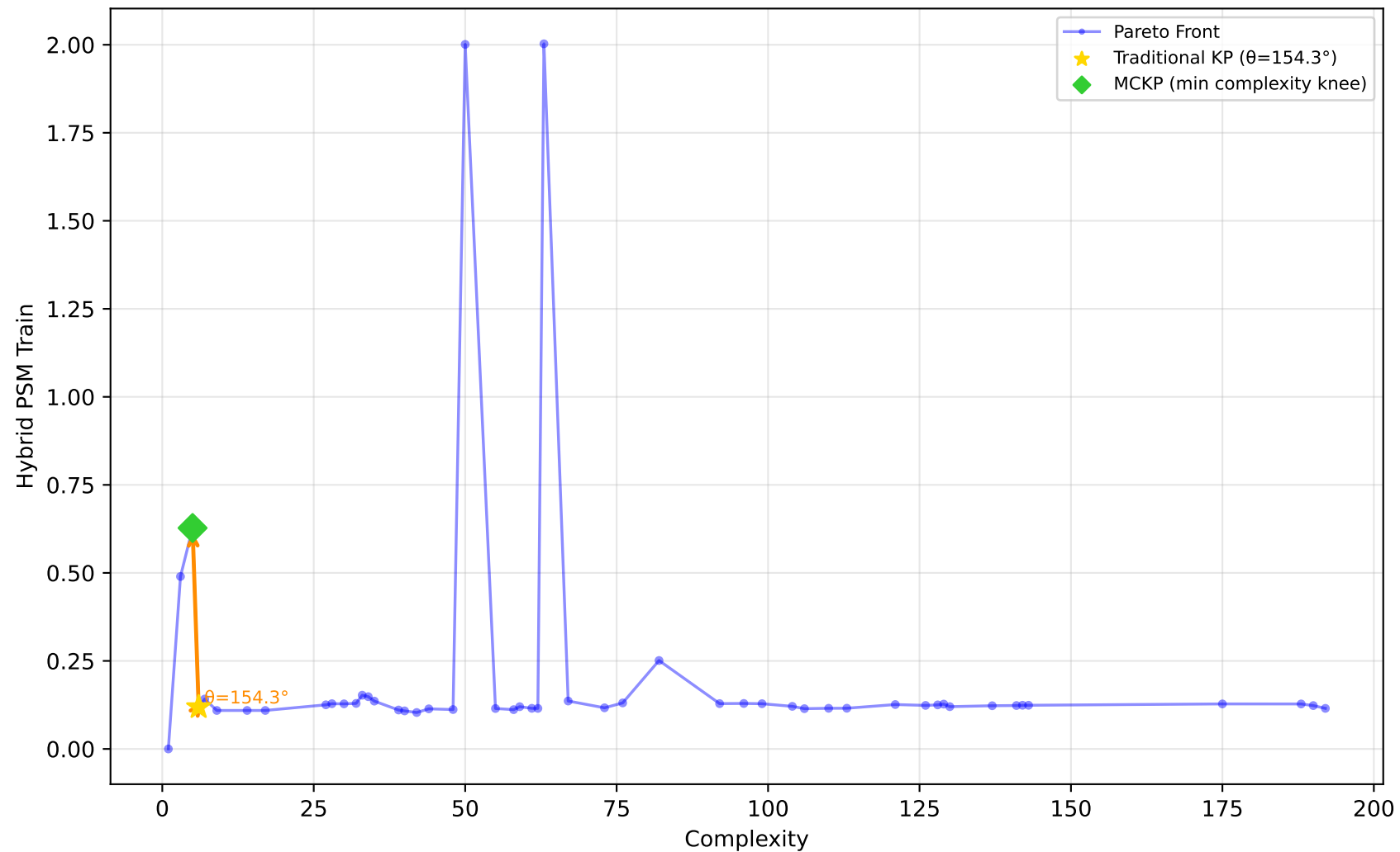
519_vinnie - Run 17 - MVP - Hybrid PSM Train \lambda_1=1.00, \lambda_2=0.00, \lambda_3=1.00 | Difficulty: 0.85 | Method: hmr
