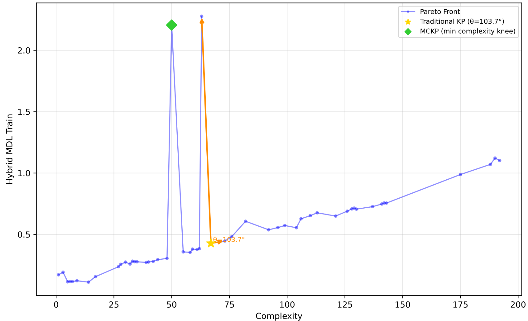
519_vinnie - Run 17 - SVP - Hybrid MDL Train \lambda_1=1.00, \lambda_2=1.00, \lambda_3=1.00 | Difficulty: 0.85 | Method: hmr
