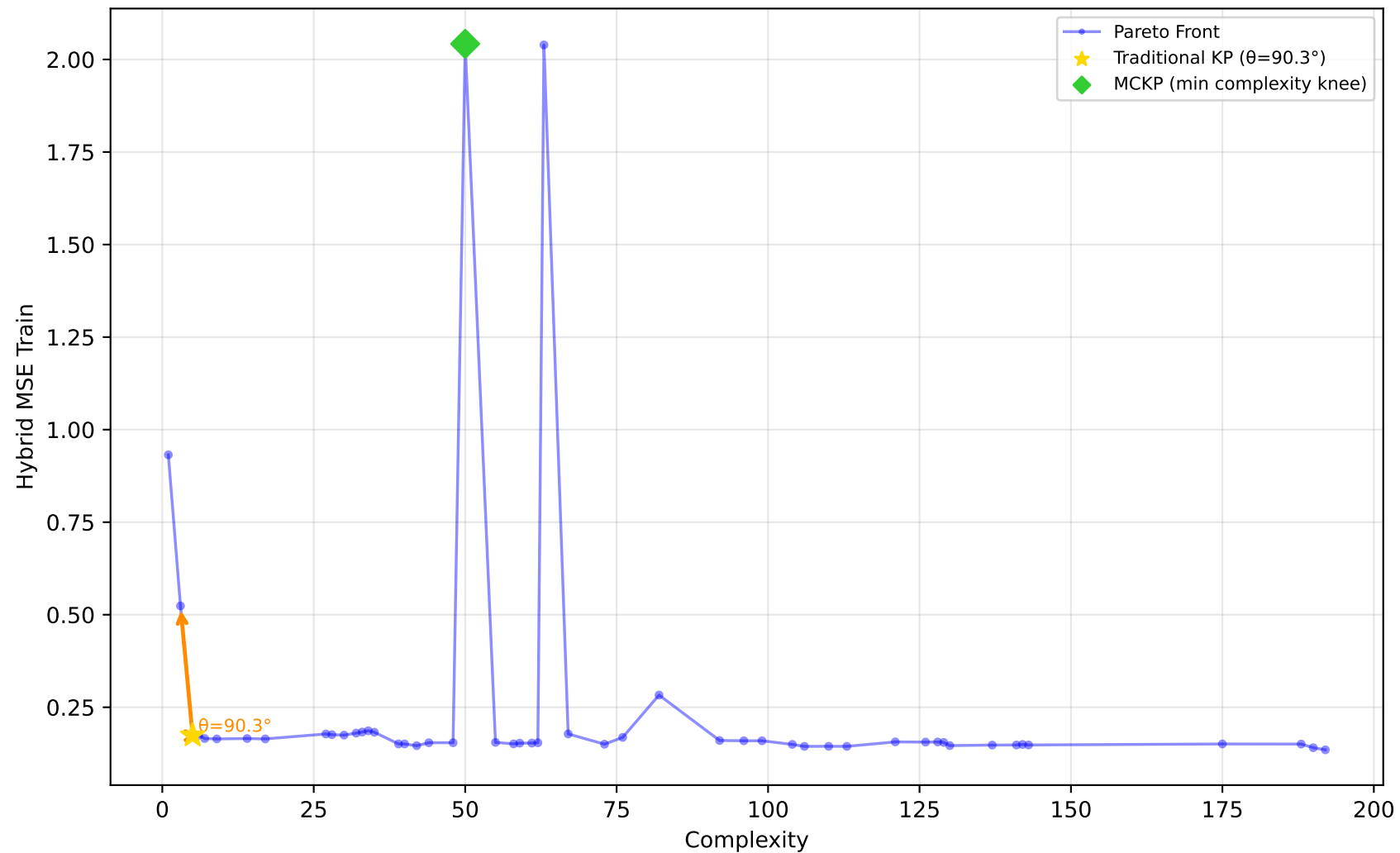
519_vinnie - Run 17 - SVP - Hybrid MSE Train \lambda_1=1.00, \lambda_2=1.00, \lambda_3=1.00 | Difficulty: 0.85 | Method: hmr
