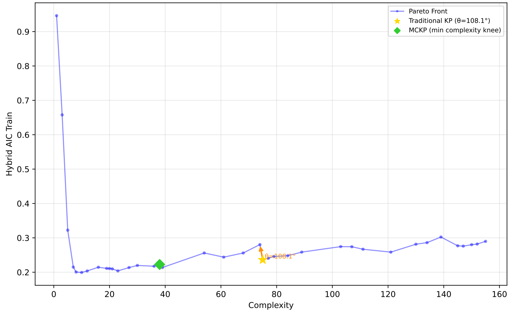
519_vinnie - Run 18 - MVP - Hybrid AIC Train \lambda_1=1.00, \lambda_2=0.00, \lambda_3=1.00 | Difficulty: 0.64 | Method: hmr
