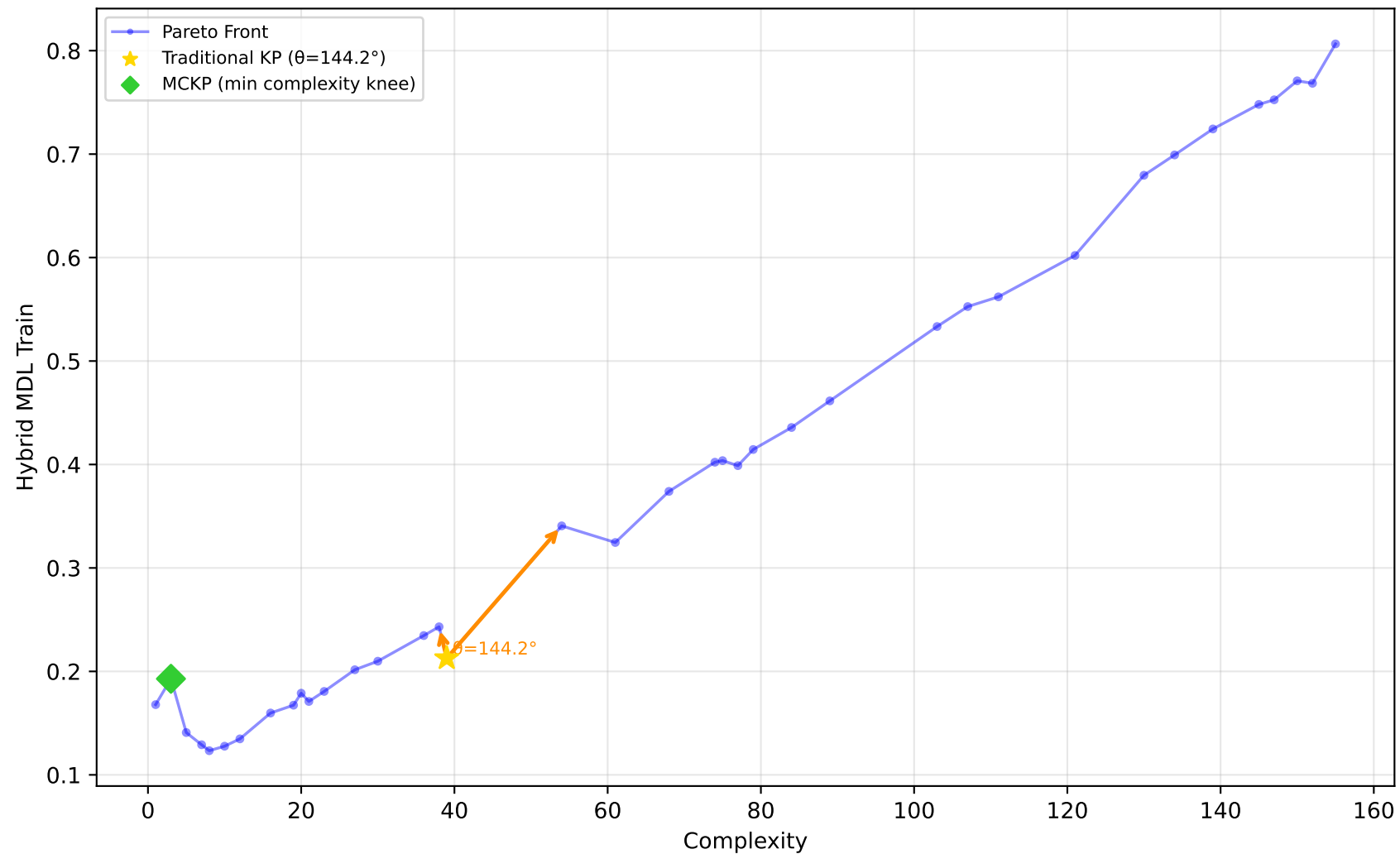
519_vinnie - Run 18 - MVP - Hybrid MDL Train \lambda_1=1.00, \lambda_2=0.00, \lambda_3=1.00 | Difficulty: 0.64 | Method: hmr
