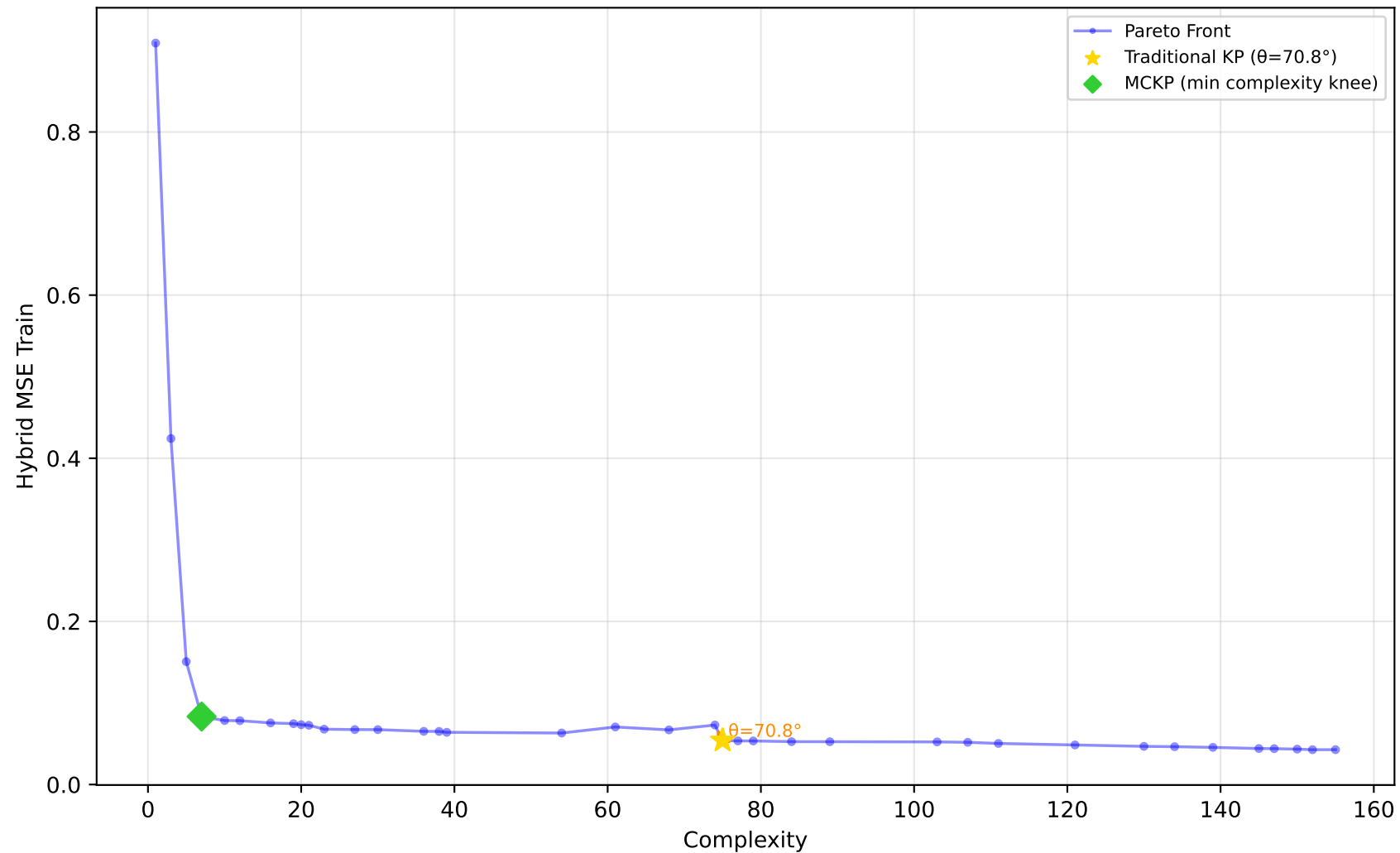
519_vinnie - Run 18 - MVP - Hybrid MSE Train \lambda_1=0.00, \lambda_2=0.10, \lambda_3=0.00 | Difficulty: 0.64 | Method: hmr
