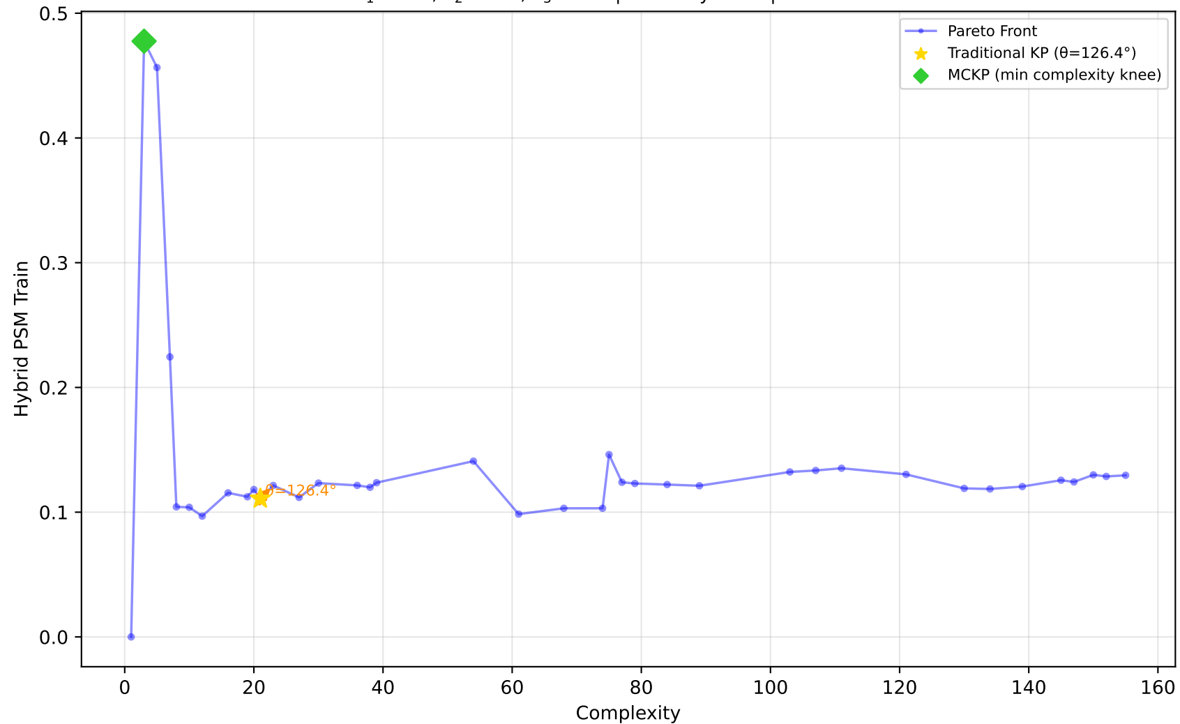
519_vinnie - Run 18 - MVP - Hybrid PSM Train \lambda_1=1.00, \lambda_2=0.00, \lambda_3=1.00 | Difficulty: 0.64 | Method: hmr
