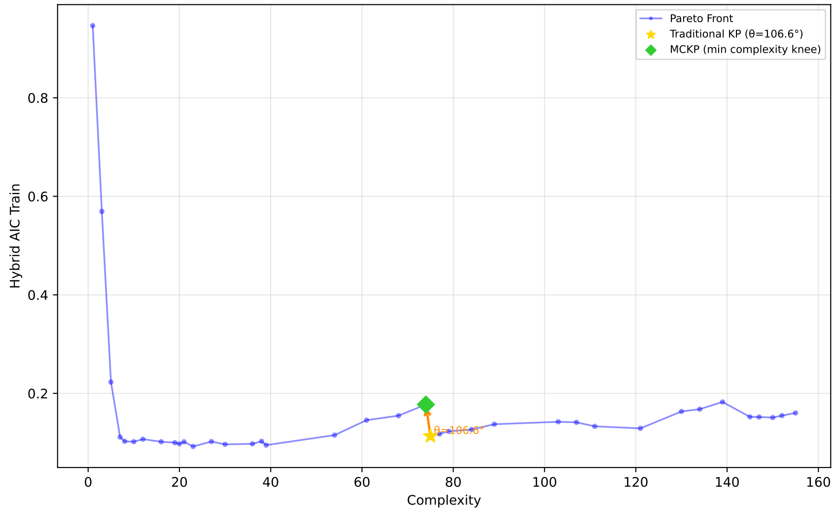
519_vinnie - Run 18 - SVP - Hybrid AIC Train \lambda_1=0.00, \lambda_2=0.00, \lambda_3=0.00 | Difficulty: 0.64 | Method: hmr
