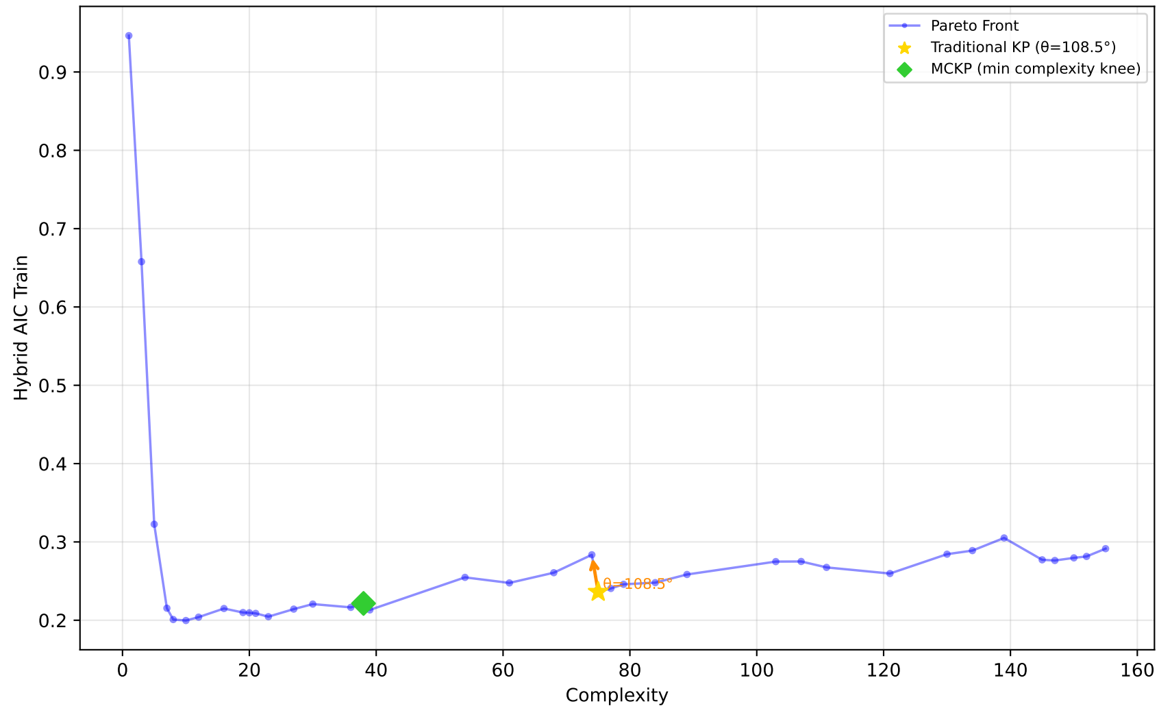
519_vinnie - Run 18 - SVP - Hybrid AIC Train \lambda_1=1.00, \lambda_2=1.00, \lambda_3=1.00 | Difficulty: 0.64 | Method: hmr
