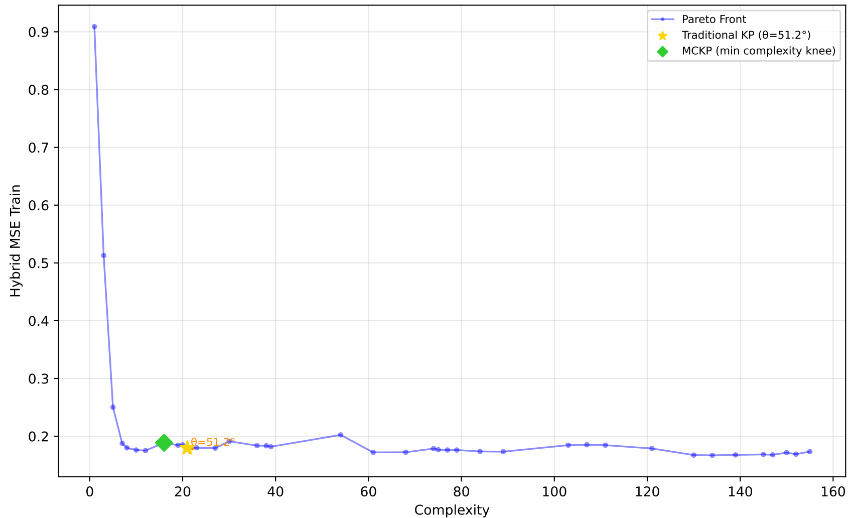
519_vinnie - Run 18 - SVP - Hybrid MSE Train \lambda_1=1.00, \lambda_2=1.00, \lambda_3=1.00 | Difficulty: 0.64 | Method: hmr
