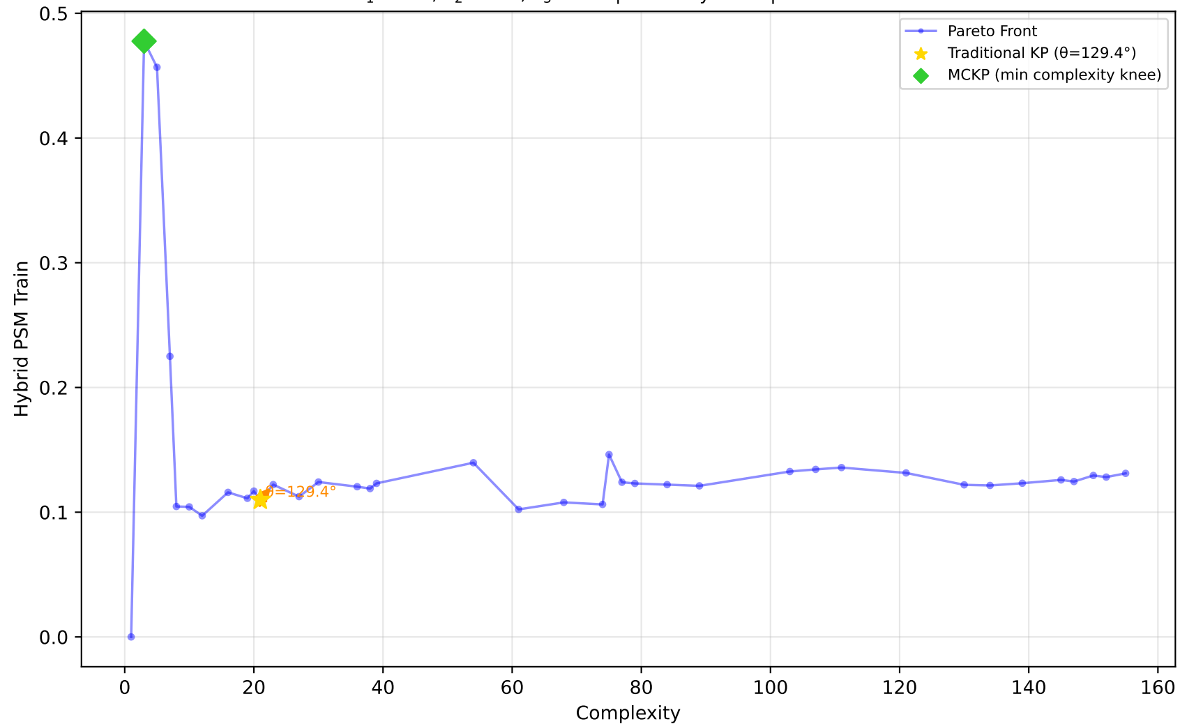
519_vinnie - Run 18 - SVP - Hybrid PSM Train \lambda_1=1.00, \lambda_2=1.00, \lambda_3=1.00 | Difficulty: 0.64 | Method: hmr
