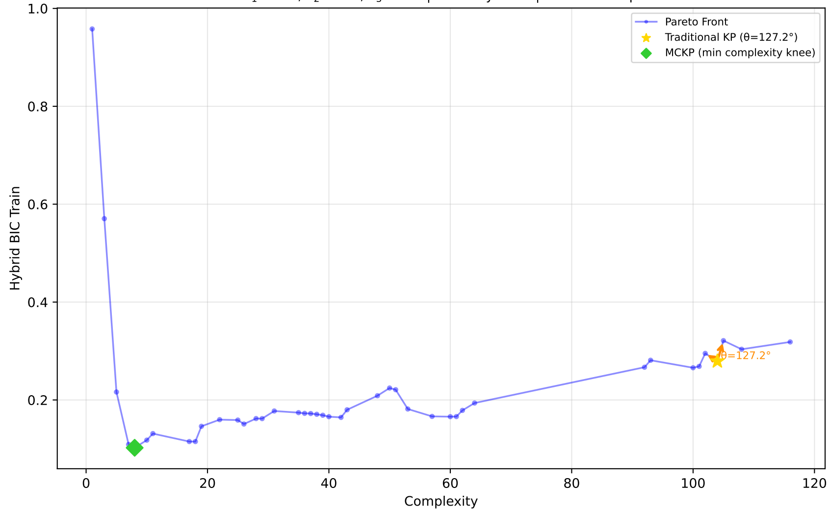
519_vinnie - Run 19 - MVP - Hybrid BIC Train \lambda_1=0.00, \lambda_2=0.10, \lambda_3=0.00 | Difficulty: 0.46 | Method: mckp
