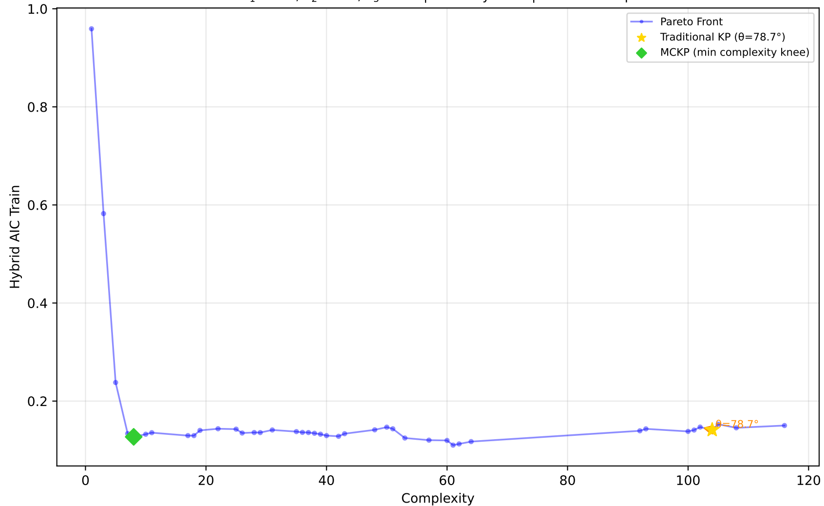
519_vinnie - Run 19 - SVP - Hybrid AIC Train \lambda_1=0.00, \lambda_2=0.00, \lambda_3=0.00 | Difficulty: 0.46 | Method: mckp
