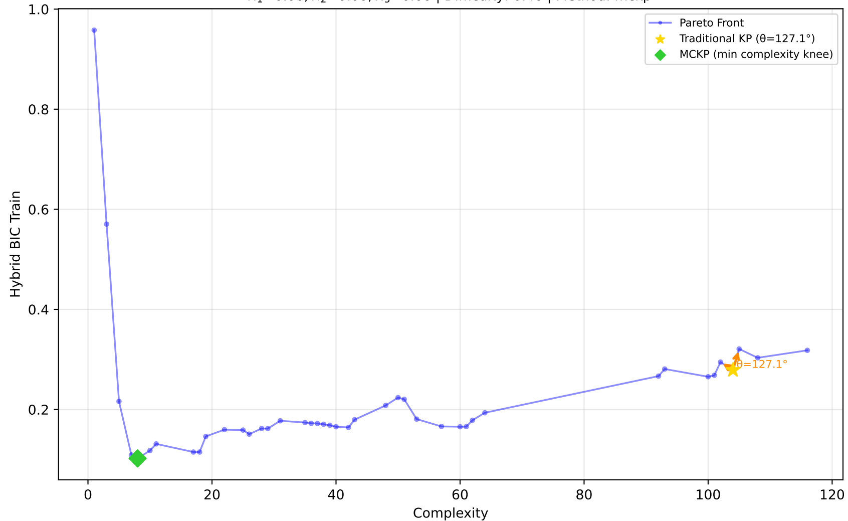
519_vinnie - Run 19 - SVP - Hybrid BIC Train \lambda_1=0.00, \lambda_2=0.00, \lambda_3=0.00 | Difficulty: 0.46 | Method: mckp
