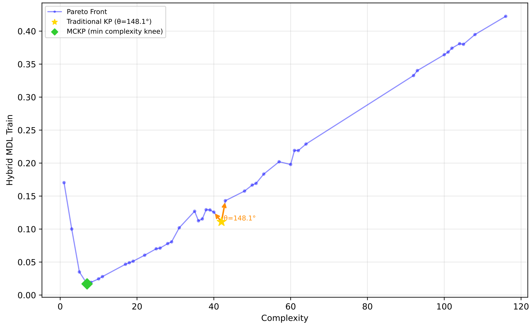
519_vinnie - Run 19 - SVP - Hybrid MDL Train \lambda_1=0.00, \lambda_2=0.00, \lambda_3=0.00 | Difficulty: 0.46 | Method: mckp
